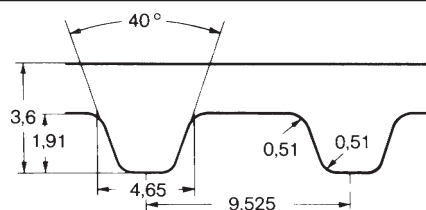
Type L
