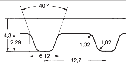
Type H
